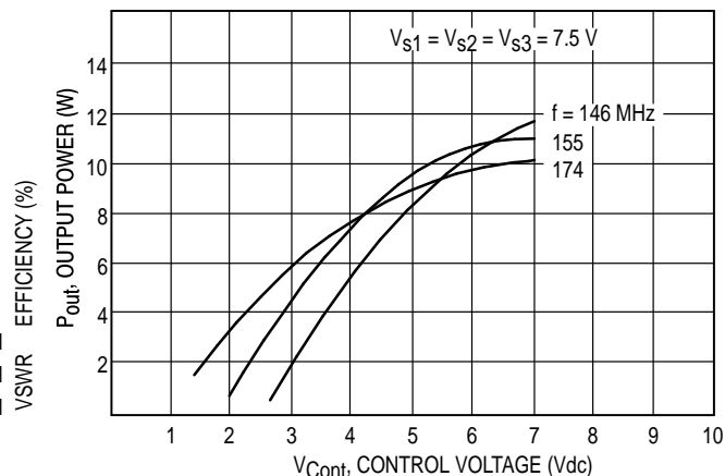
Figure 3. Output Power versus Control Voltage
